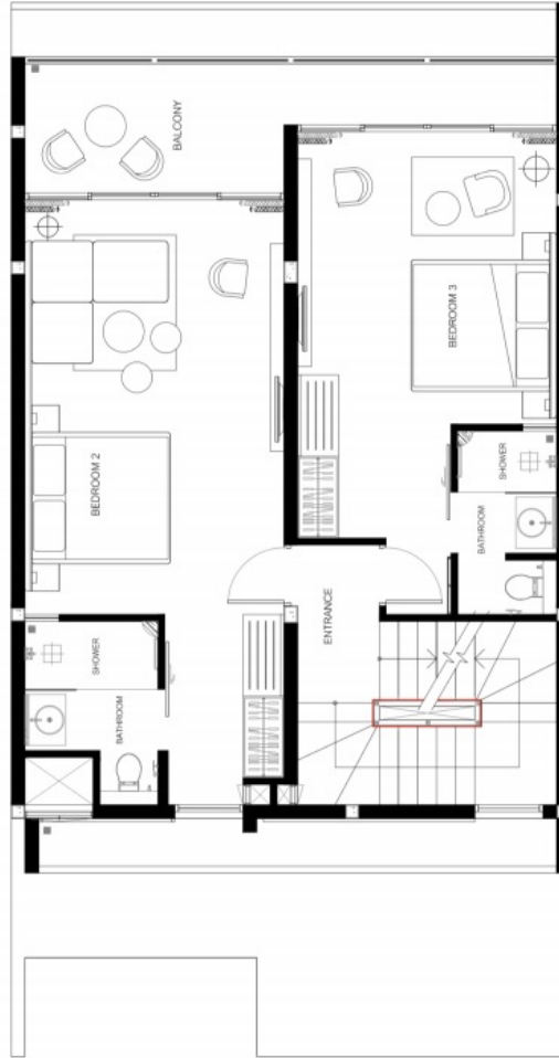
VILLA 2ND FLOOR PLAN SCALE
