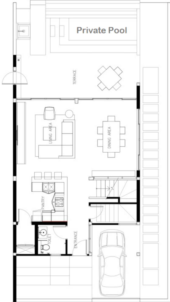
VILLA GROUND FLOOR PLAN SCALE
